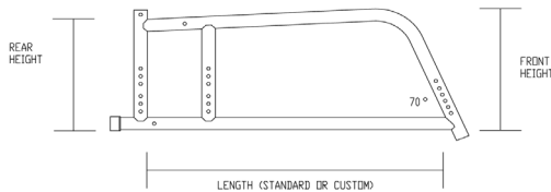
Frame Dimensions
