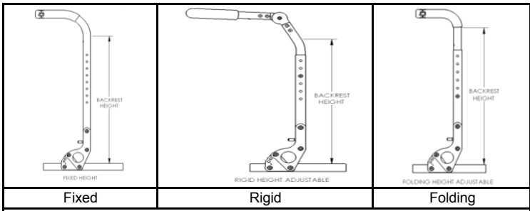
FIGURE 9.1 - HANDLE HEIGHT DIAGRAMS
