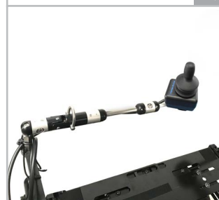
Link-It to Midline Swing-Away Joystick Mount
