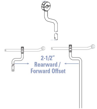
ONYX REARWARD OFF-SET VERTICAL ROD
