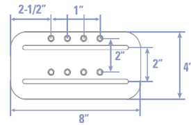
SLIDE MOUNT
